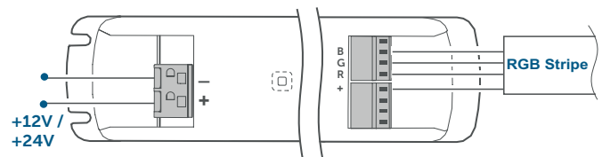
RGB strip connection
