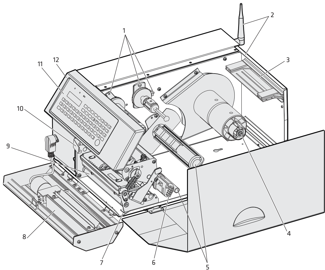
PX6i Spare Parts Overview
