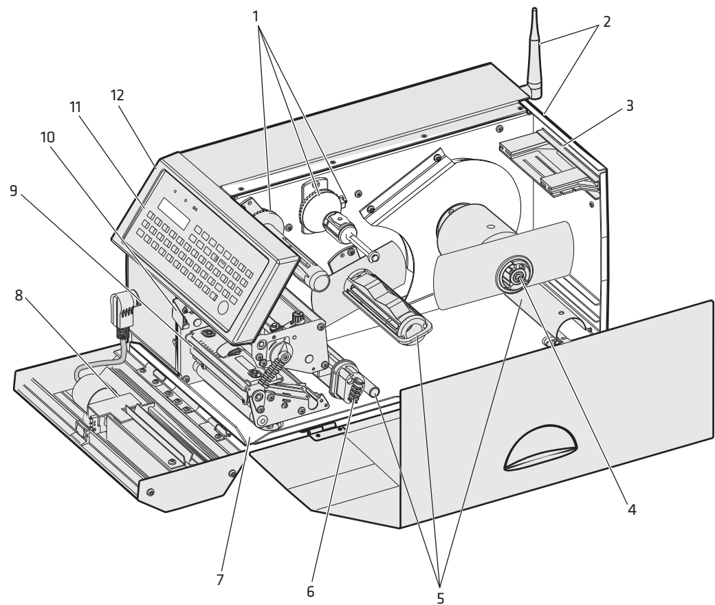
PX4i Spare Parts Overview
