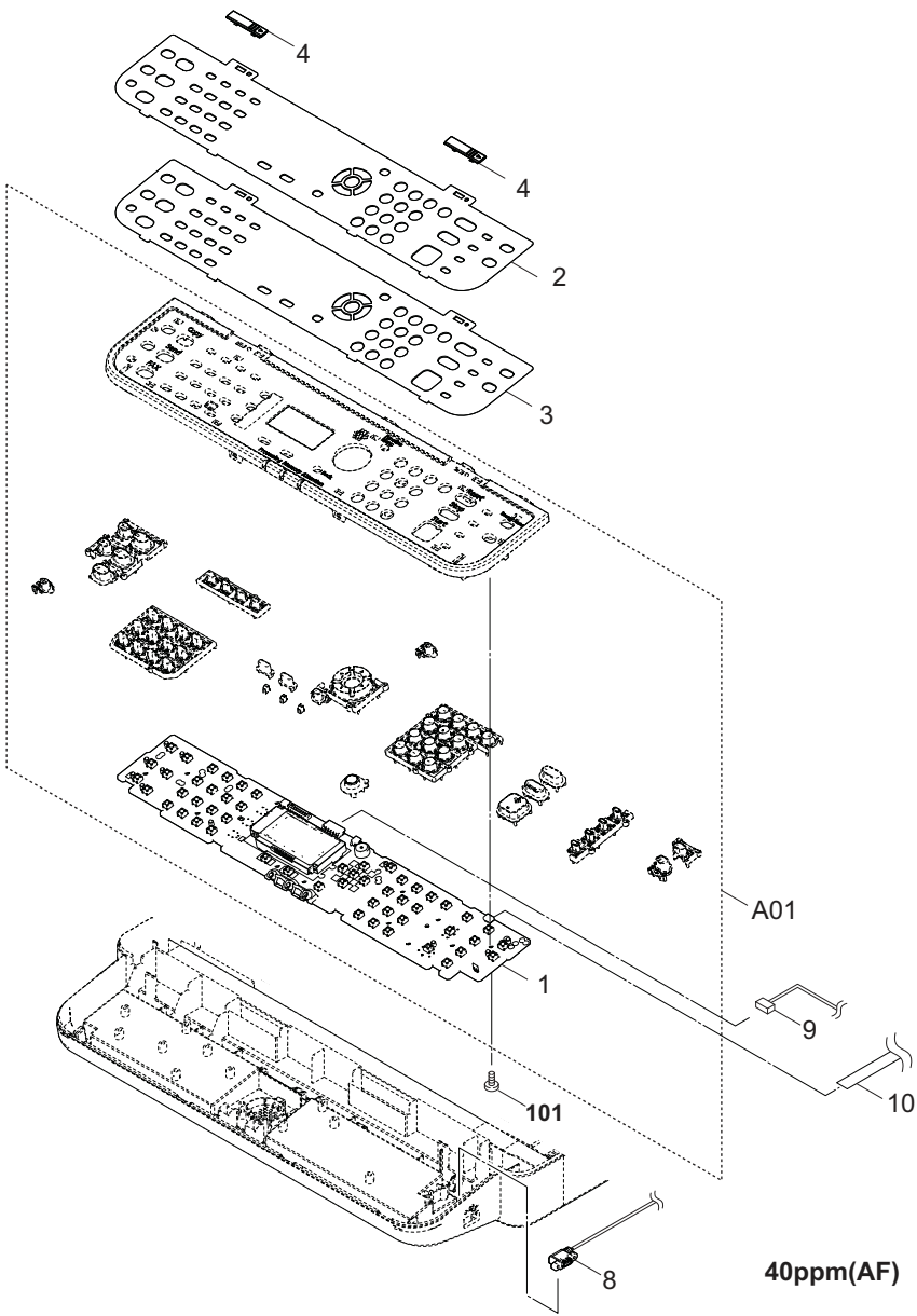
FIG. 11 Operation Section(40ppm(A)/40ppm(AF))
