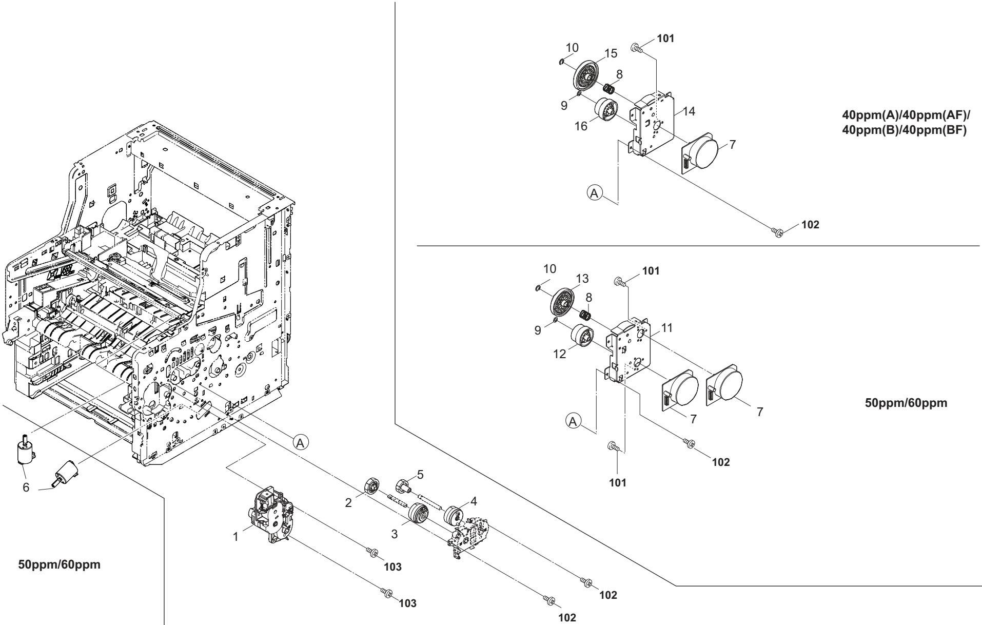
FIG. 10 Drive Section
