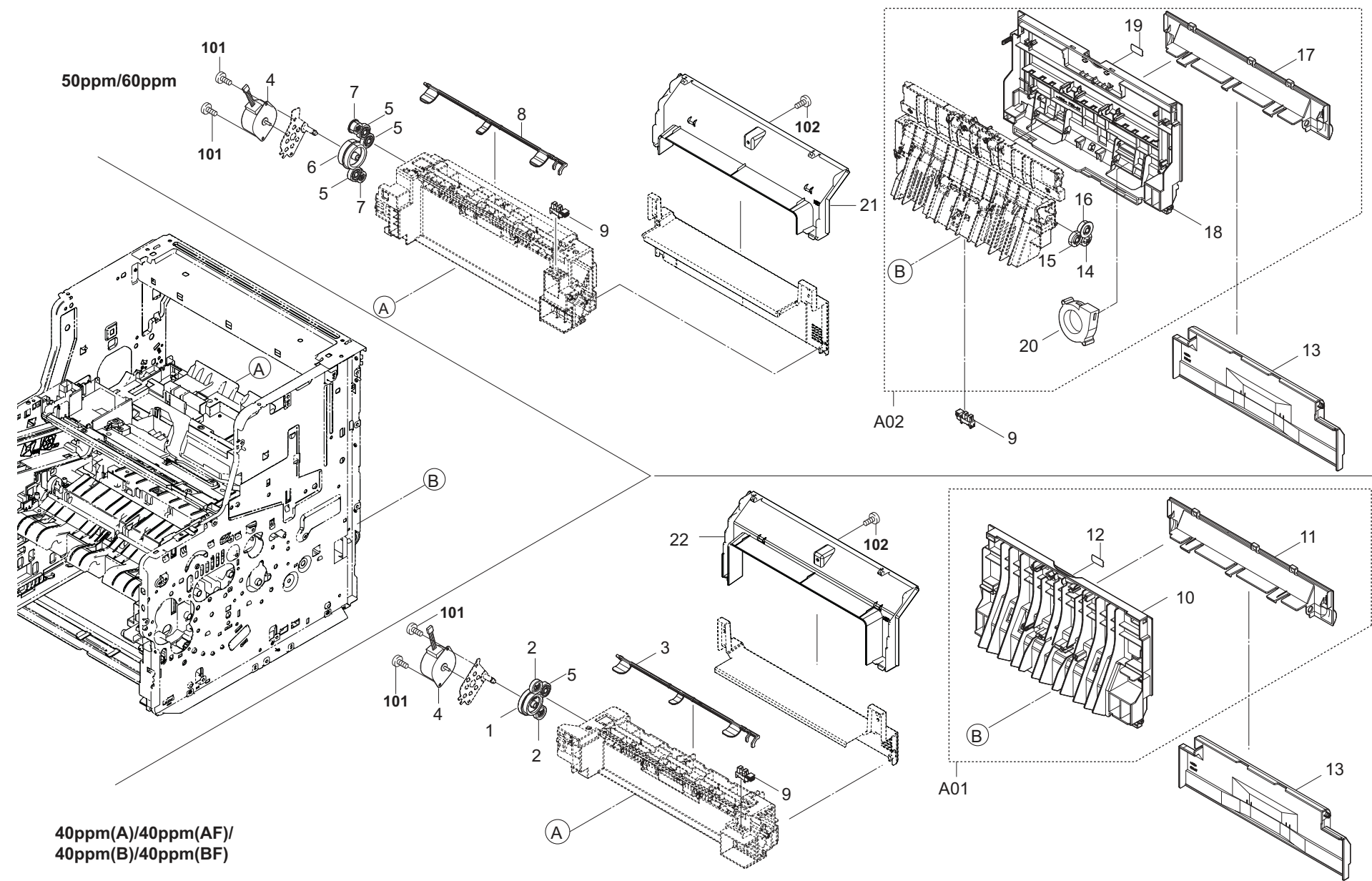
FIG. 8 Exit Section
