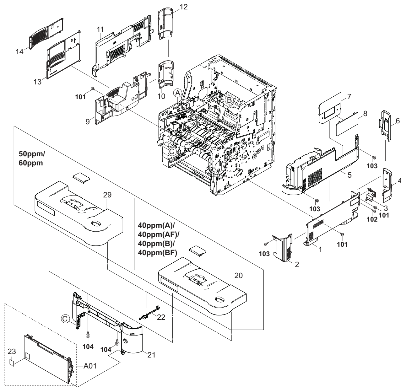
FIG. 1 Covers
