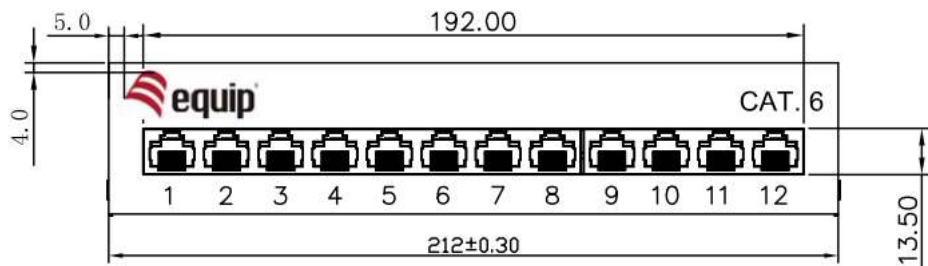
Plan View
