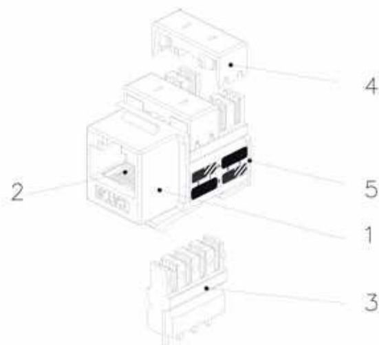
110/KRONE DUAL IDC
