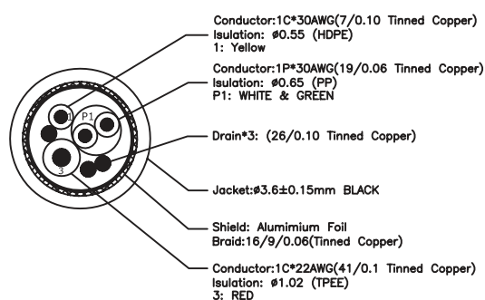
CABLE Cross Section.:
