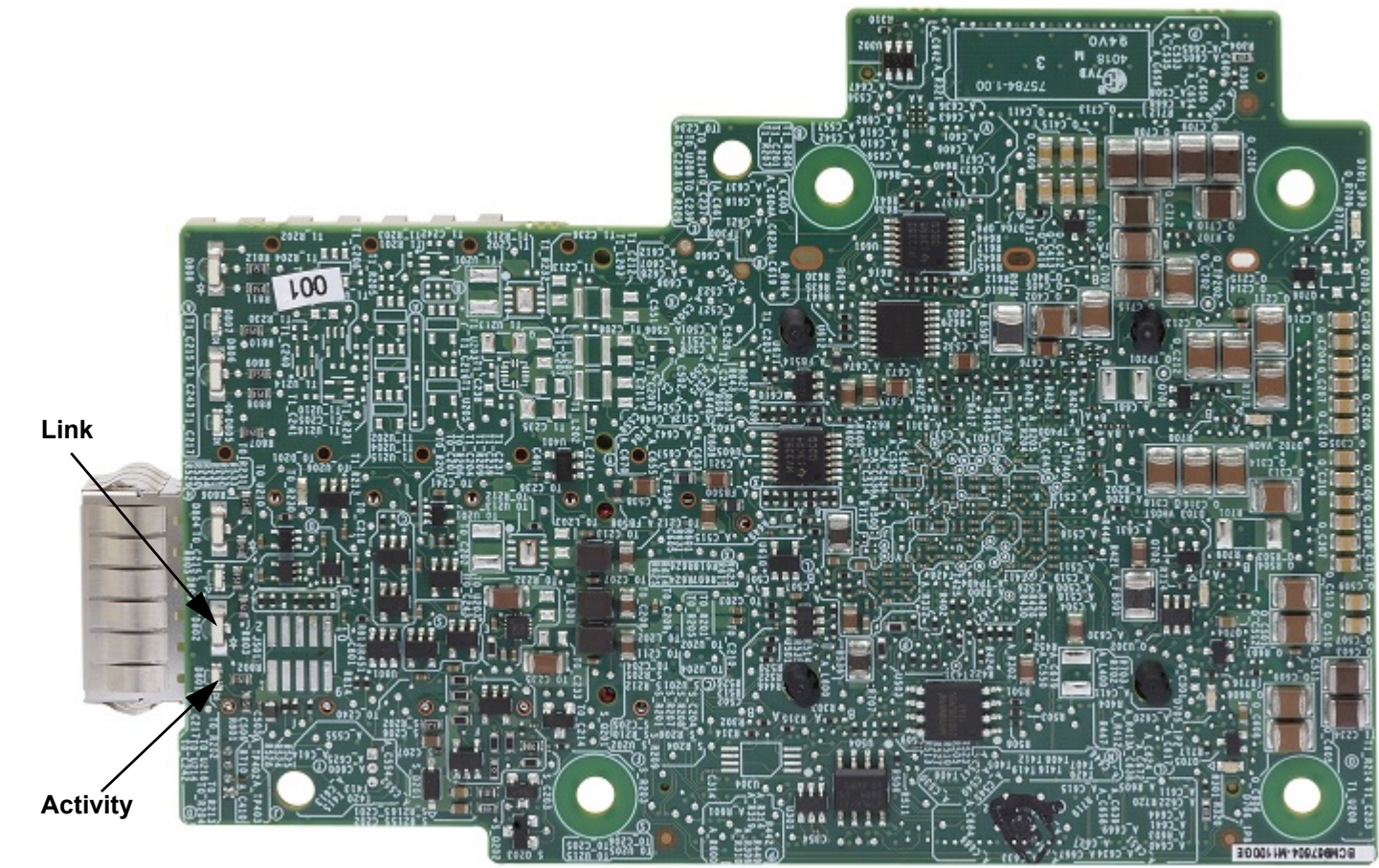
Figure 4: Activity and Link LED Locations
