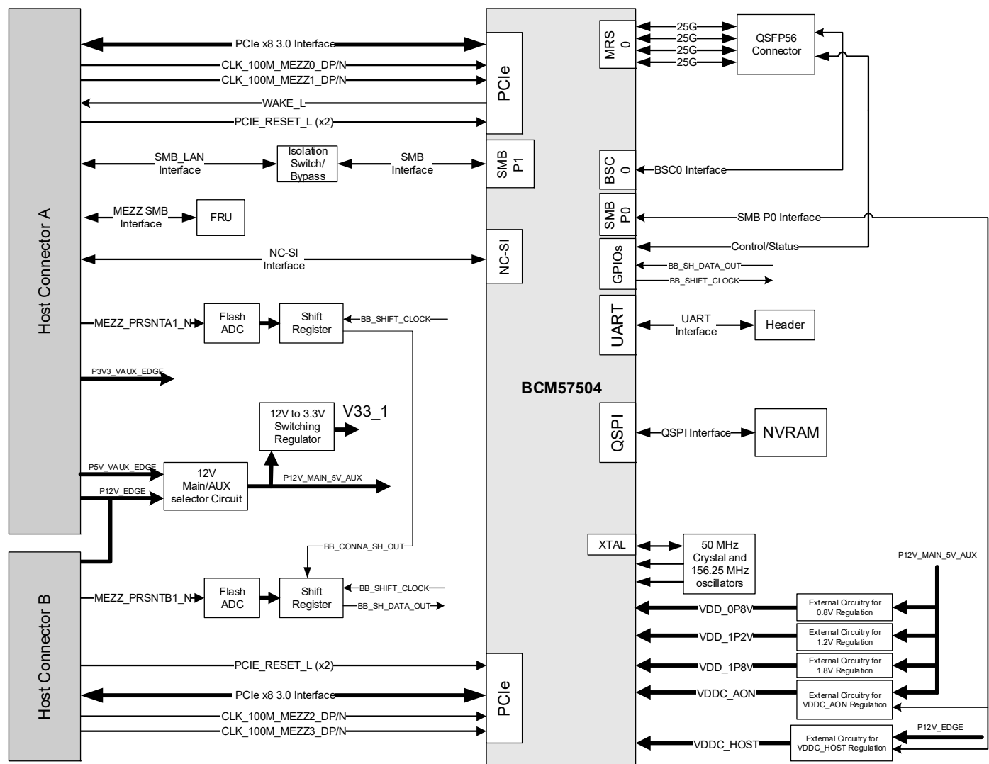
Figure 2: BCM957504-M1100G16 Block Diagram
