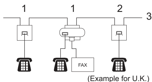
Figure 1: Inadvisable connection
