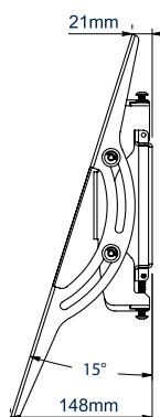
SIDE VIEWS
