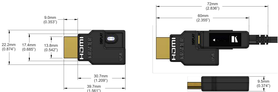
Figure 2: HDMI Connectors – SOURCE and DISPLAY (with Dimensions in mm)
