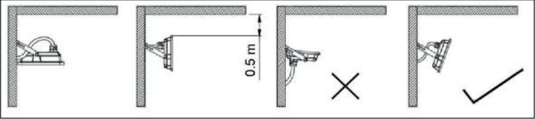
Fig. 2: Mounting
