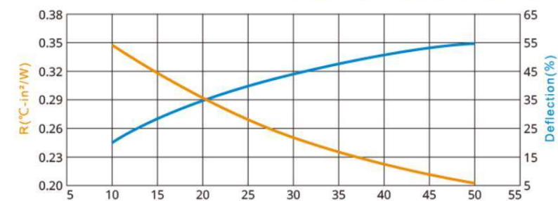
Thermal Resistance VS. Pressure VS. Deflection
