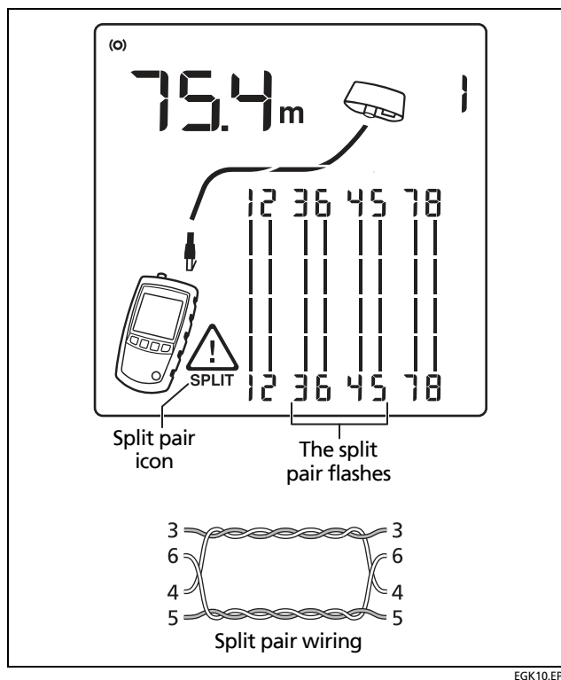
Figure 12. Split Pair
