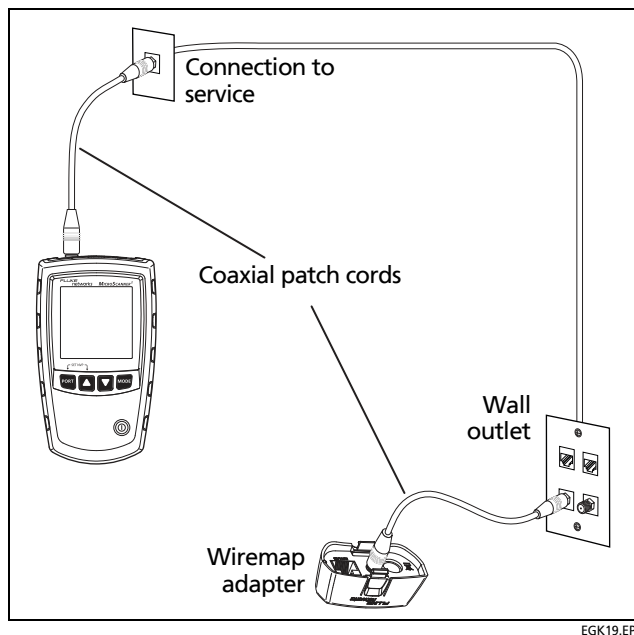
Figure 22. Connecting to Coaxial Cabling (MicroScanner 2 )
