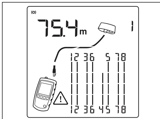
Figure 8. Open on Twisted Pair Cabling
