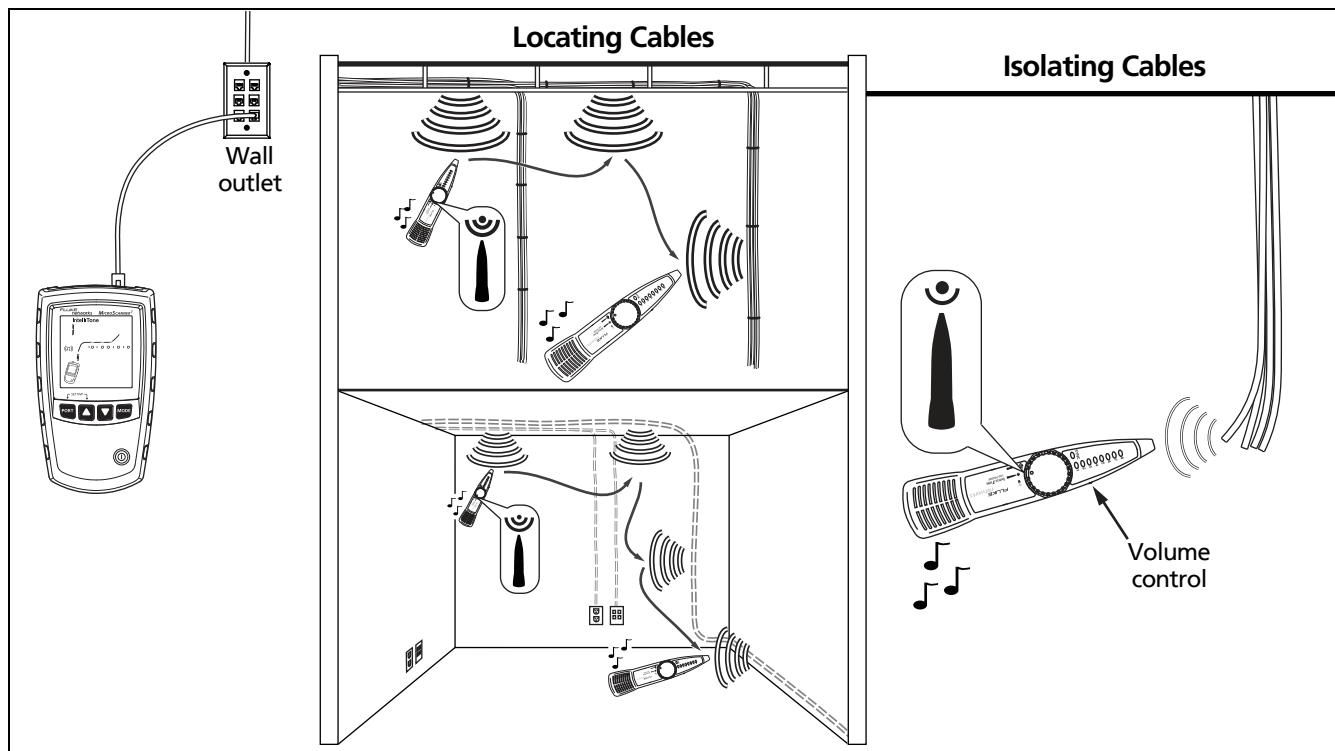
Figure 34. Using the Toner in IntelliTone Mode
