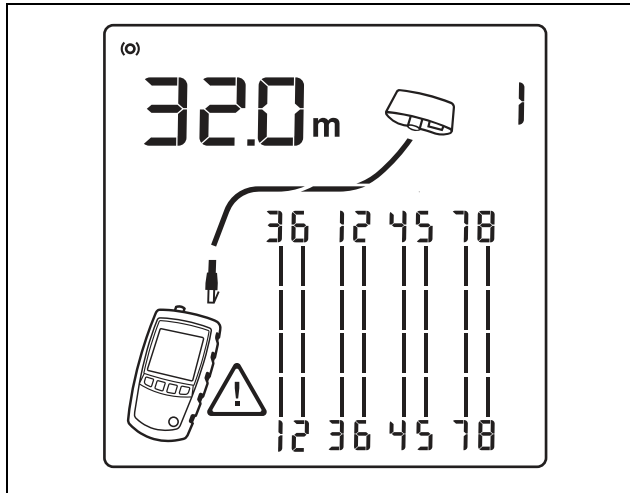
Figure 11. Crossed Pairs
