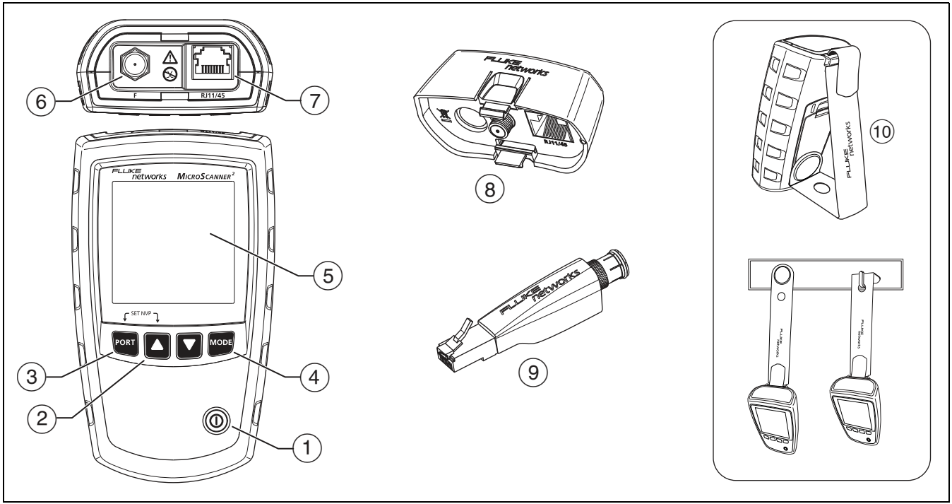
Figure 4. MicroScanner 2 Features
