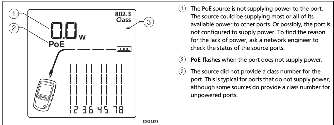
Figure 31. PoE Port that Shows 0.0 W
