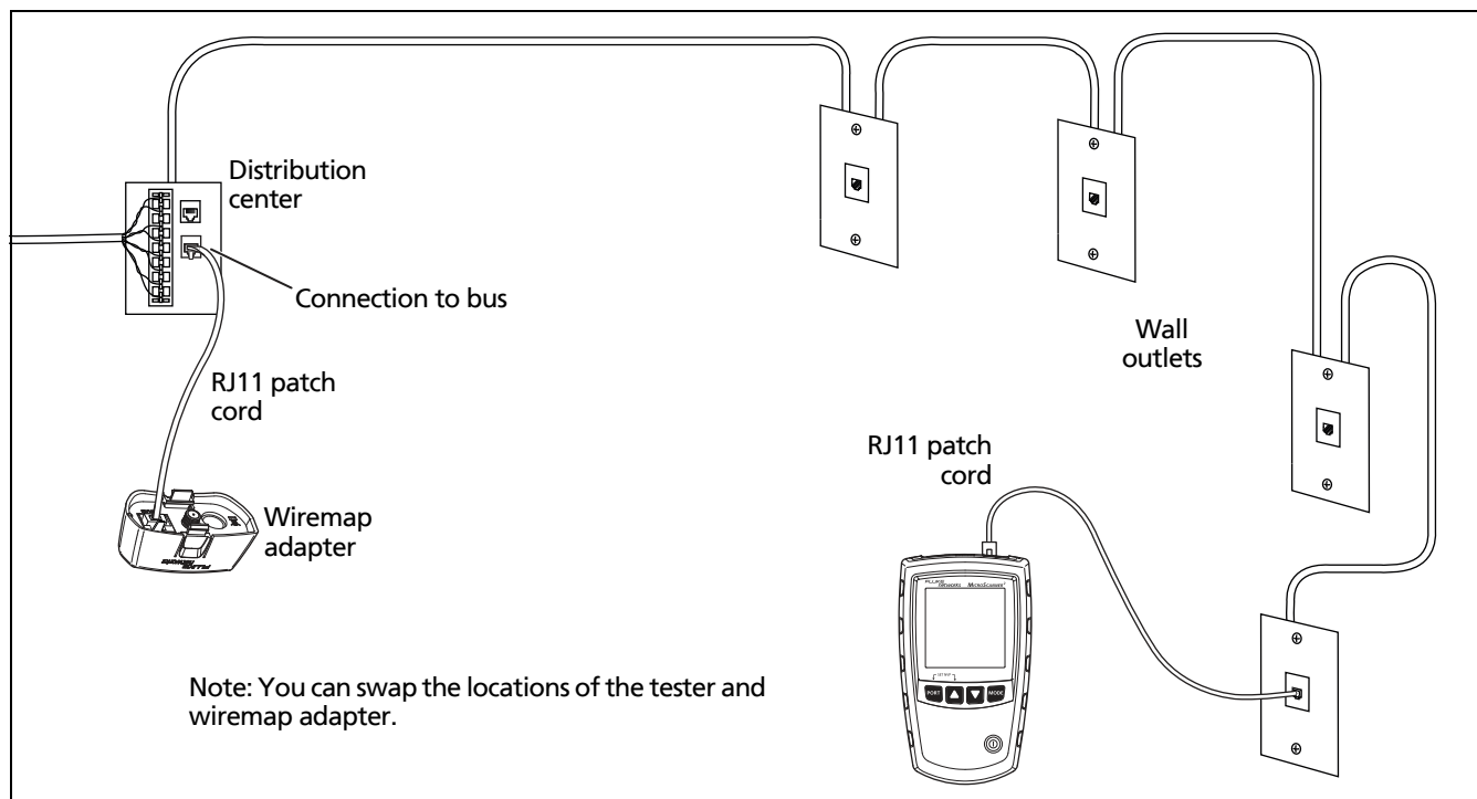
Figure 21. Connecting to a Telephone Network Wired in a Bus Topology
