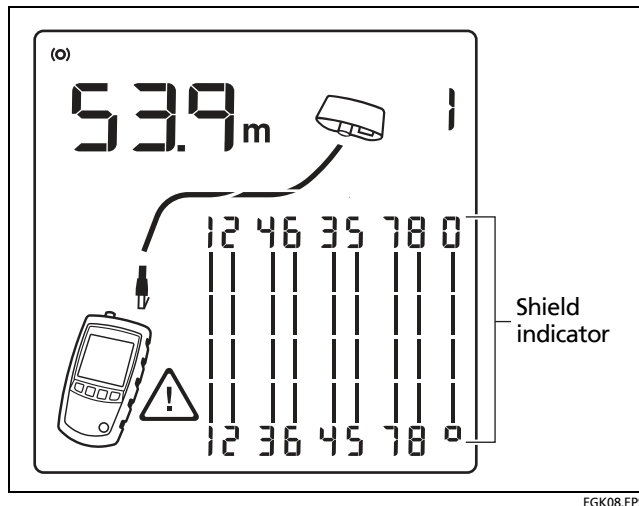
Figure 10. Crossed Wires
