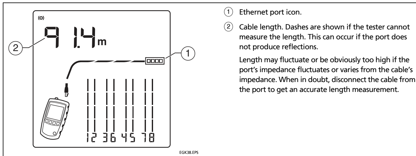
Figure 16. Inactive Ethernet Port Detected
