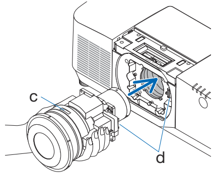
c: Plate / d: Connector
