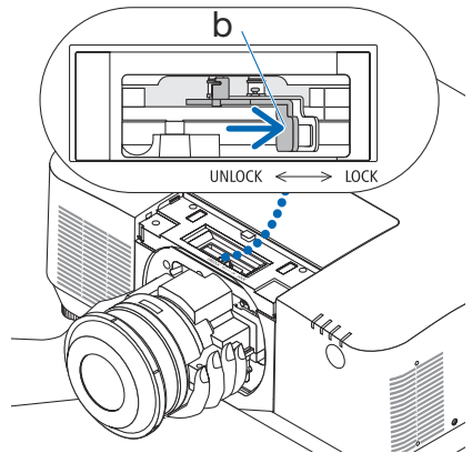
b: Lens lock lever
