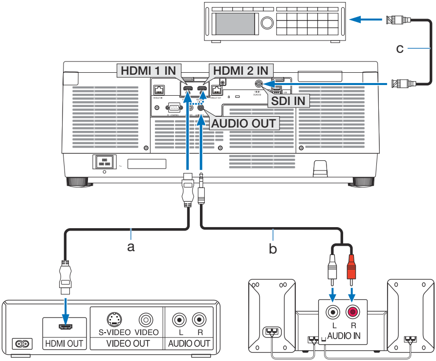
a: HDMI cable (not supplied) (Use a Premium High Speed HDMI Cable.) / b: Audio cable (not supplied) / c: BNC cable (not supplied)
