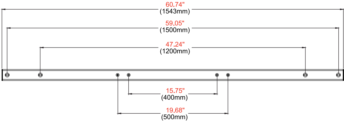
FRONT VIEW
