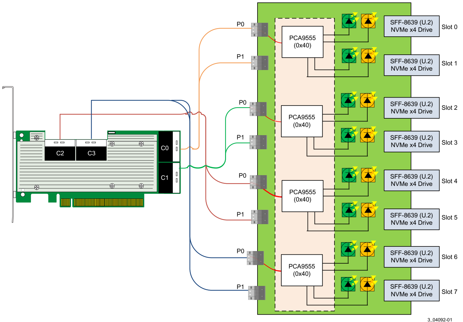
Figure 3 Backplane with x4 Connectors and VPP
