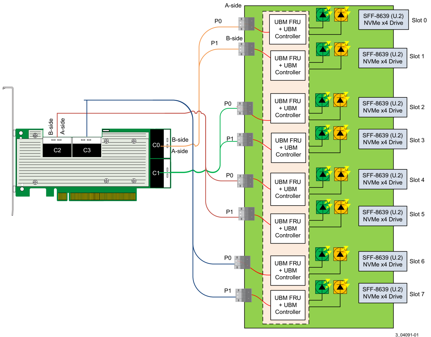
Figure 2 Backplane with x4 Connectors
