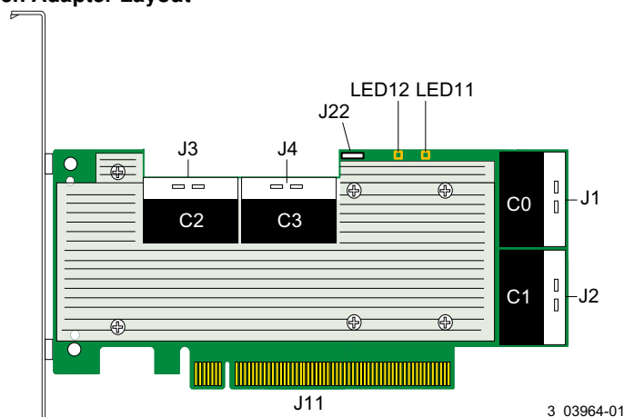
Figure 6 P411W-32P NVMe Switch Adapter Layout
