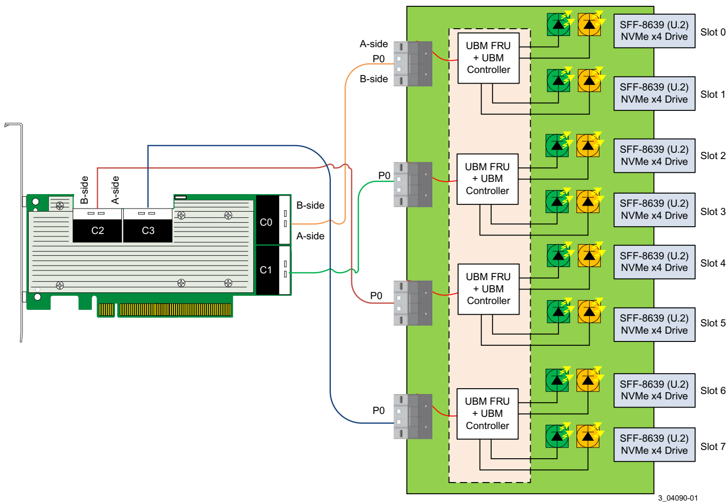
Figure 1 Backplane with x8 Connectors
