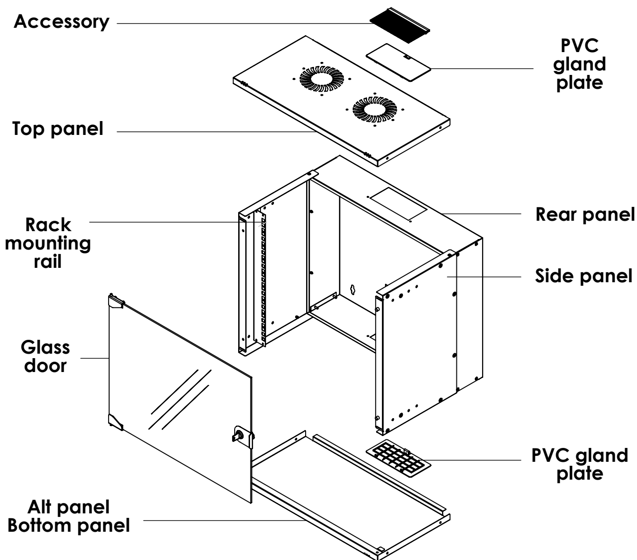
Exploded view
