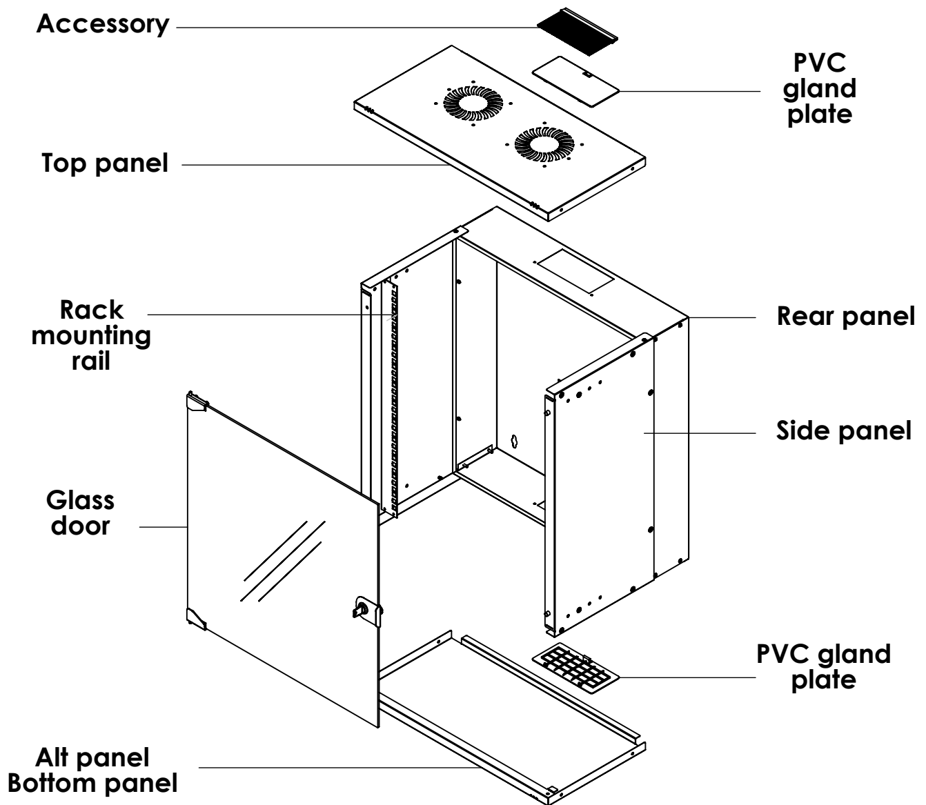
Exploded view
