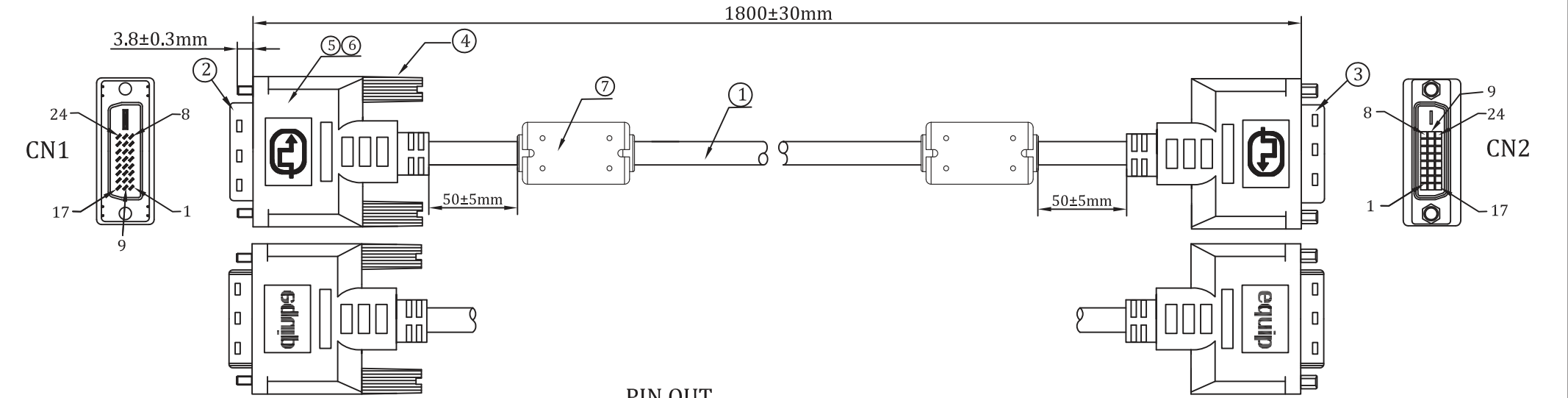
PIN OUT
