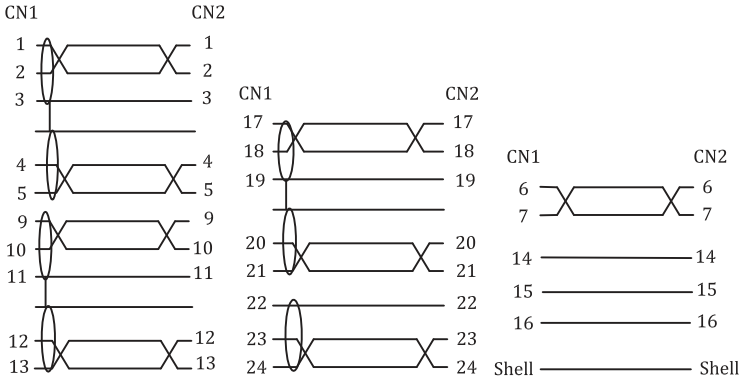
PIN OUT
