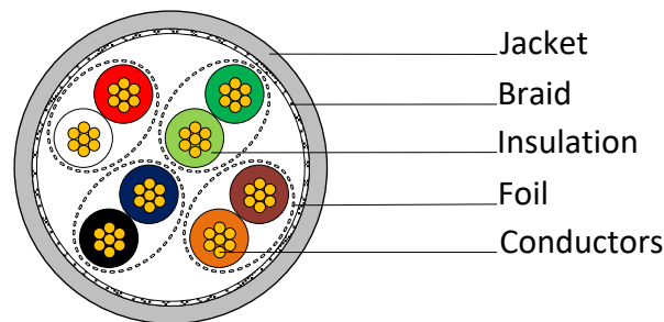
Cross section
