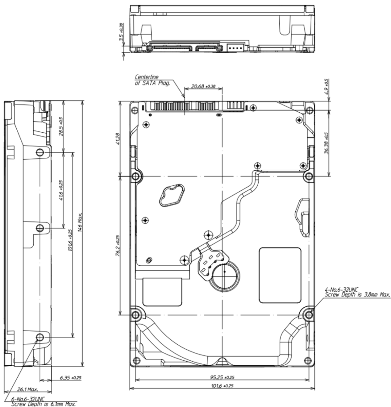
Figure 3.1 Dimensions
