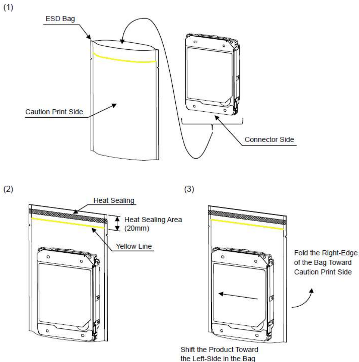
Figure 5.1 Bag packaging
