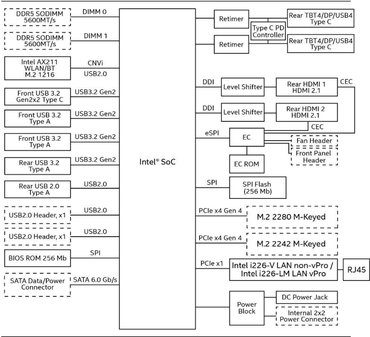
Figure 6. Block Diagram
