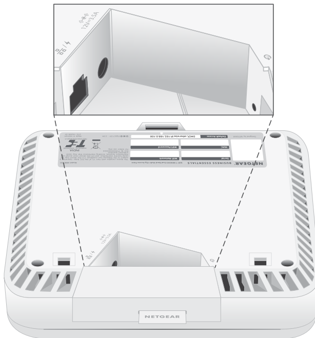
Figure 2. Hardware interfaces
