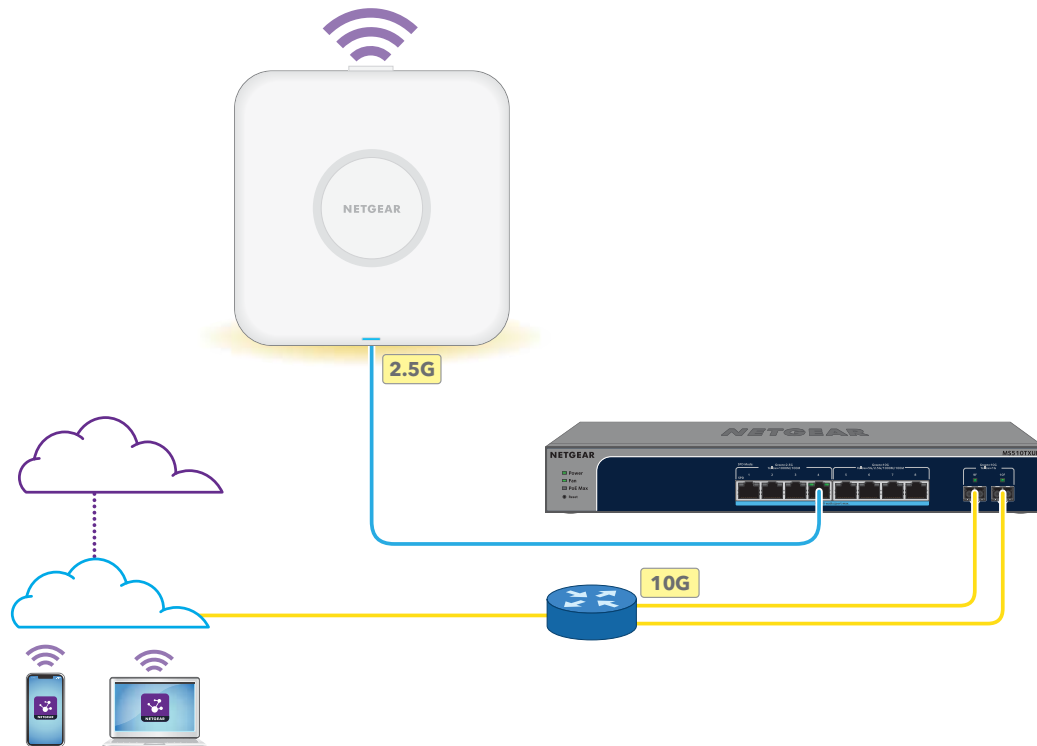
Figure 5. Set up the AP in a NETGEAR Insight configuration
