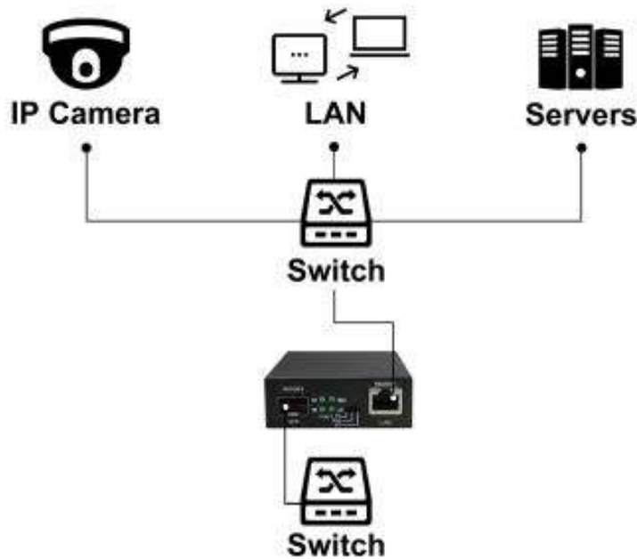
Figure 3-1 Connection schematic 1
