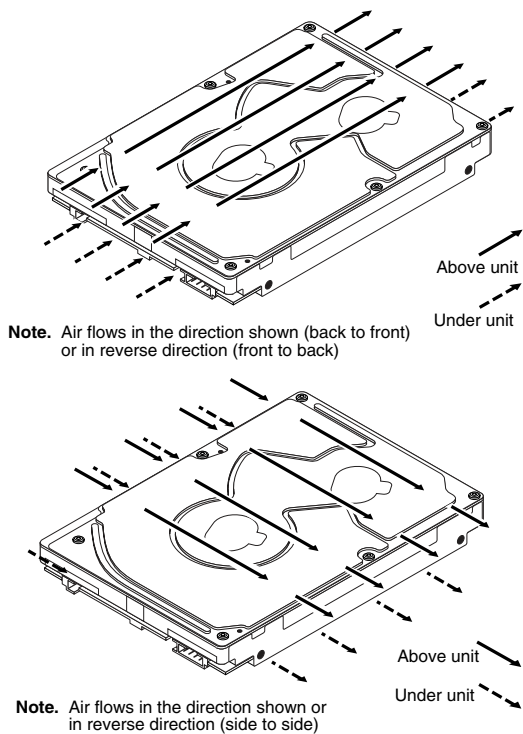
Figure 5. Air flow
