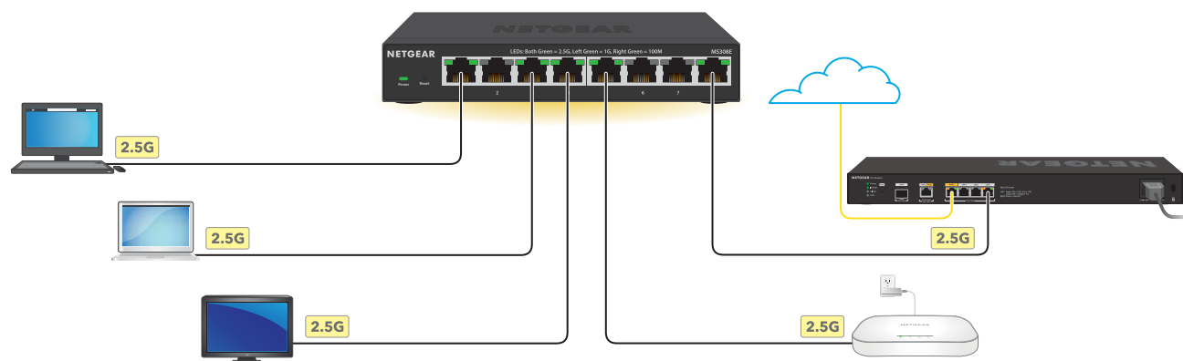
Figure 3. Example connections
