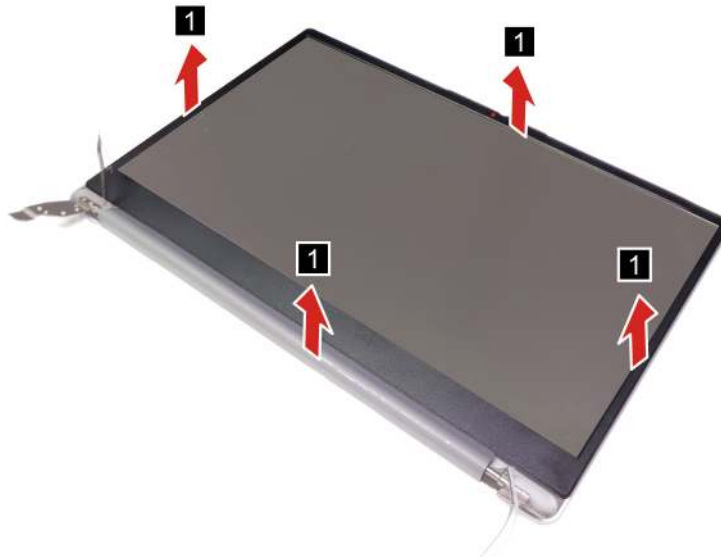
Figure 39. Remove the LCD bezel
