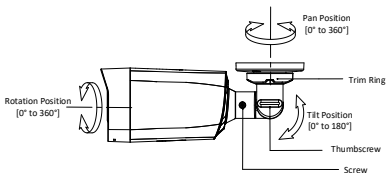
Figure 2-2 3-Axis Adjustment
