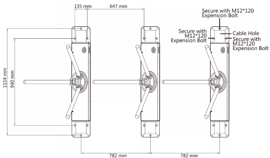
Figure 3-3 Installation Footprint
