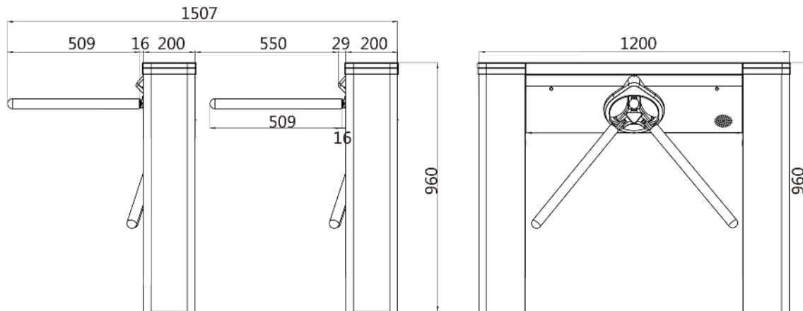
Figure 3-2 Dimension
