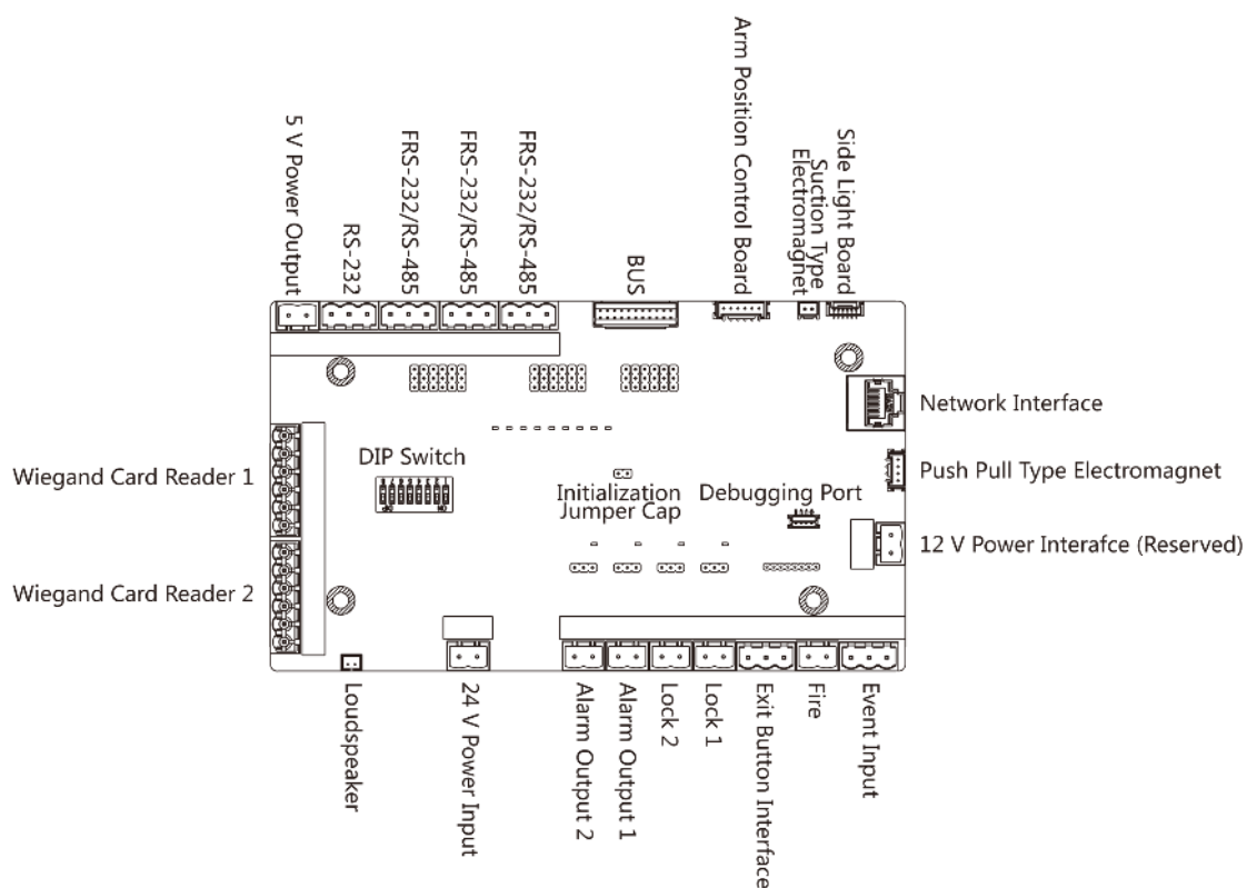
Figure 4-2 Access Control Board Diagram
