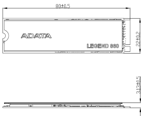
<With heatsink>
