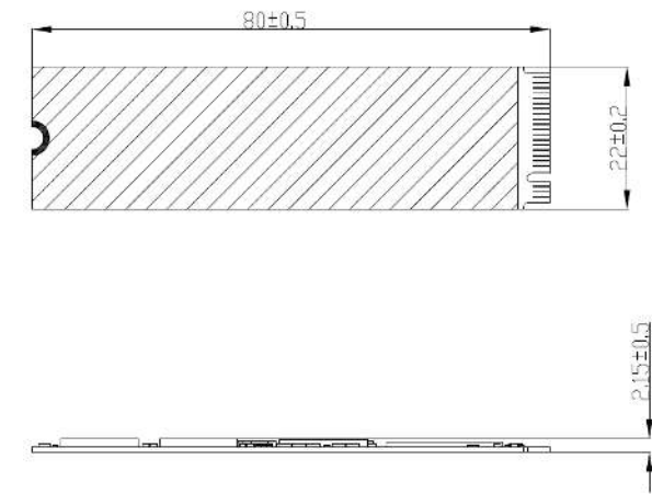
<Without heatsink>
