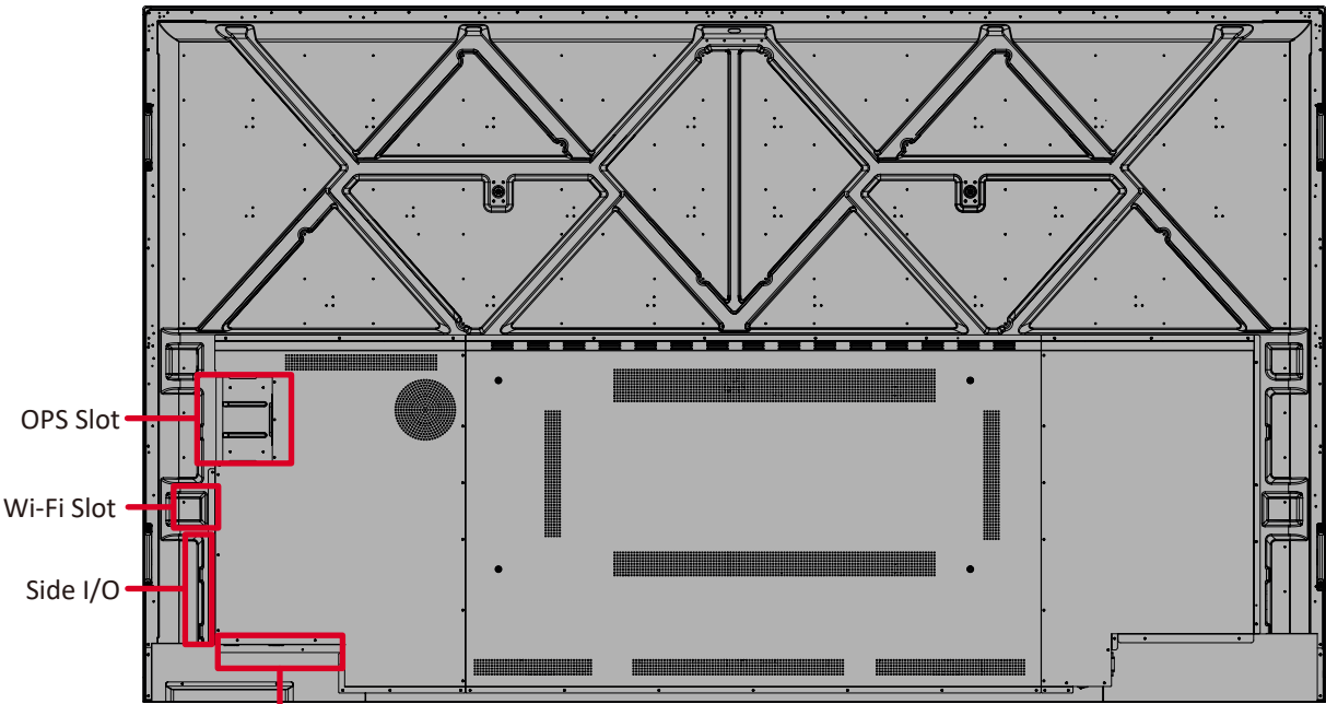
Rear I/O
