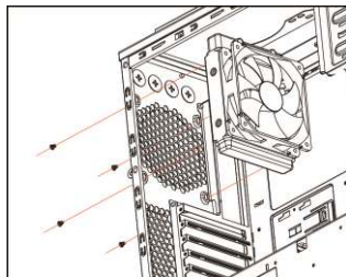
Option 1: Screw the radiator to the fixed rear fan position.
