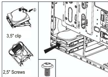
Pull out HDD tray
