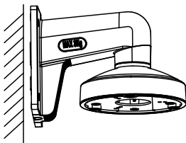
Figure 2-22 Fix the Wall Mount
