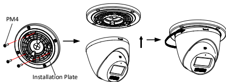
Figure 2-20 Fix the Camera to the Junction Box Cover
