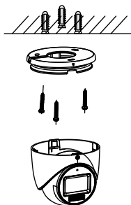
Figure 2-7 Secure the Base to the Ceiling
