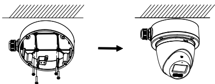
Figure 2-21 Fix the Junction Box Cover and Junction Box Body
