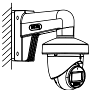
Figure 2-17 Finish the Installation
