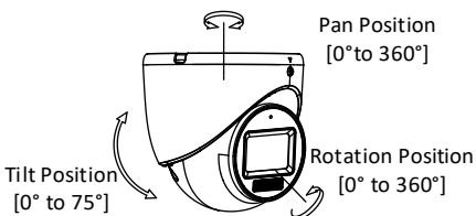
Figure 2-9 3-Axis Adjustment
