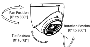
Figure 2-19 3-Axis Adjustment
