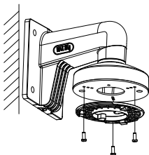
Figure 2-23 Fix the Installation Plate
