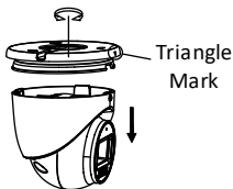
Figure 2-15 Disassemble the Camera
