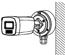
Figure 2-5 Fix the Cover to Its Body
