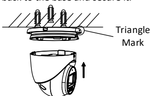
Figure 2-8 Install the Camera Back
