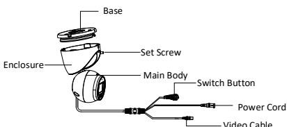
Figure 1-3 Overview of Type III Camera
