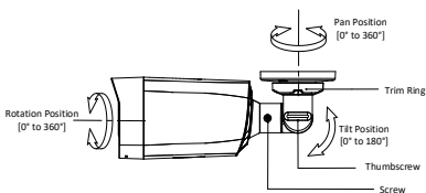
Figure 2-2 3-Axis Adjustment
