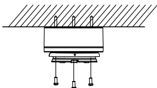
Figure 2-12 Fix the Base
