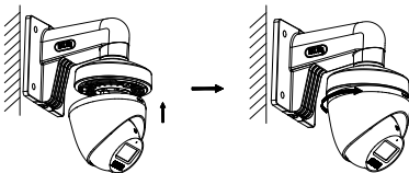
Figure 2-24 Finish Installation
