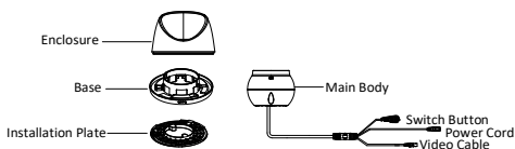
Figure 1-5 Overview of Type V Camera
