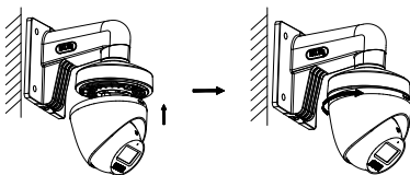
Figure 2-24 Finish Installation
