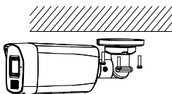
Figure 2-1 Secure the Camera to the Ceiling
