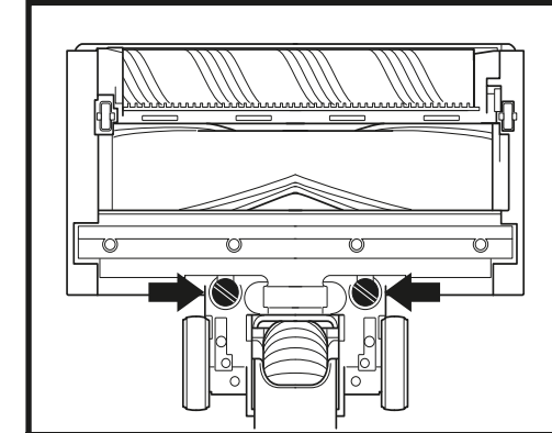
REMOVING SQUEEGEE
