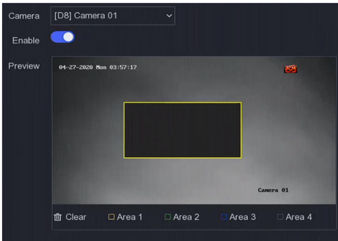
Figure 6-13 Privacy Mask
