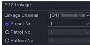
Figure 6-21 PTZ Linkage
