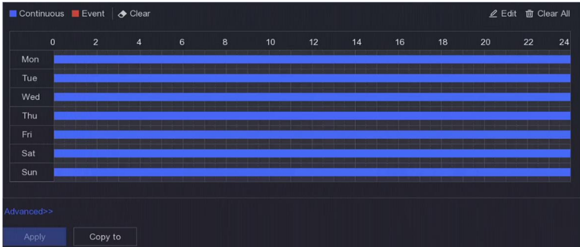
Figure 6-22 Recording Schedule
