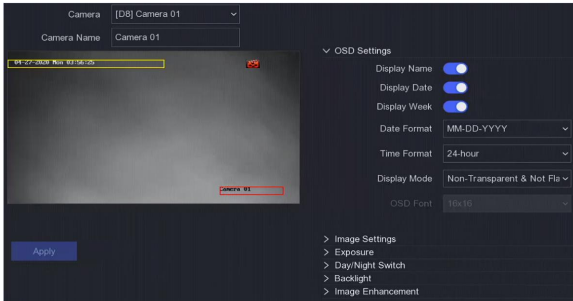
Figure 6-12 OSD
