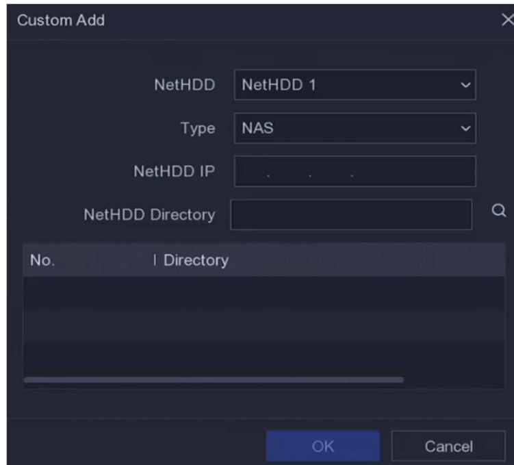
Figure 6-23 Add NetHDD
