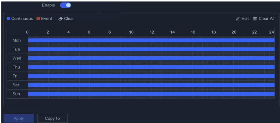
Figure 5-10 Recording Schedule
