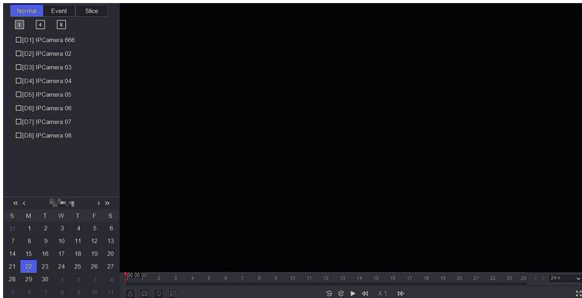
Figure 3-1 Playback
