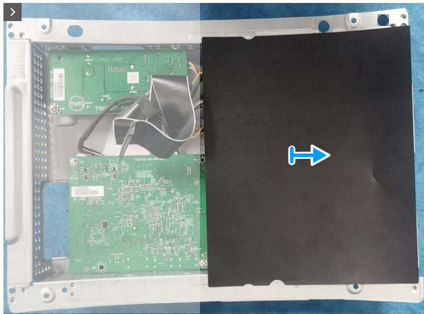
Figure 30. Removing the system board and power board
