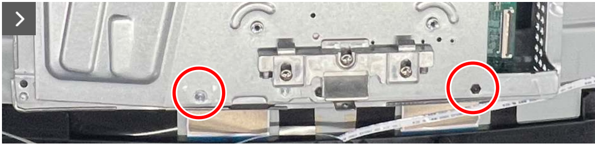
Figure 23. Removing the metal shield
