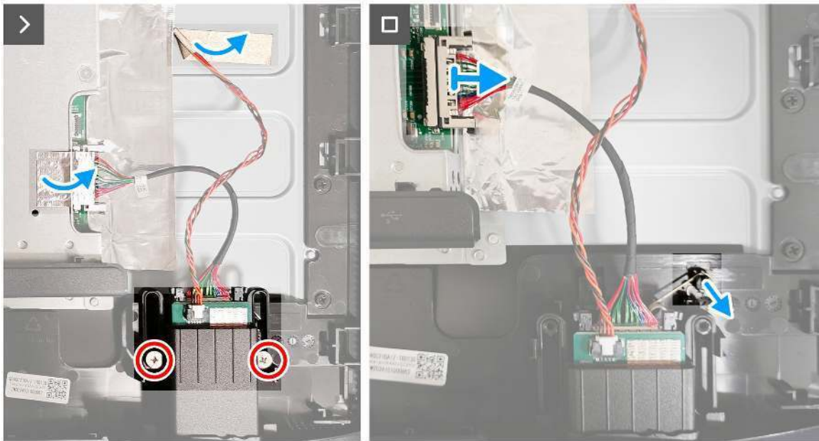
Figure 19. Removing the USB hub
