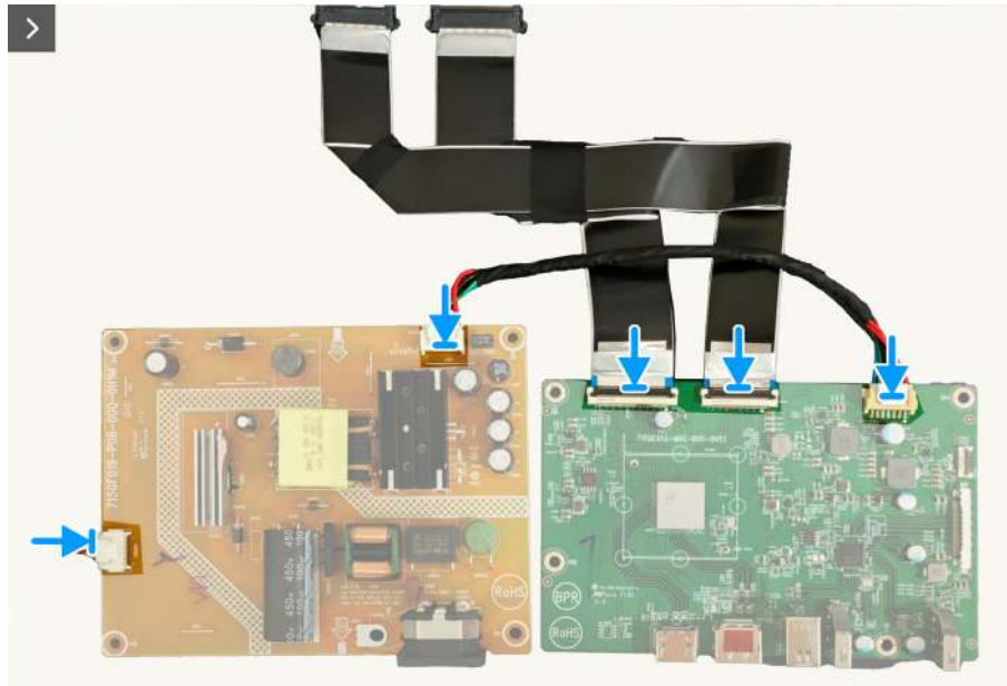
Figure 28. Installing the system board and power board
