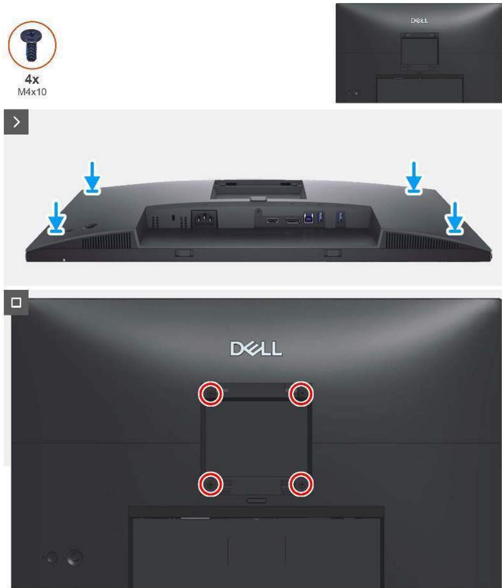
Figure 14. Installing the back cover
