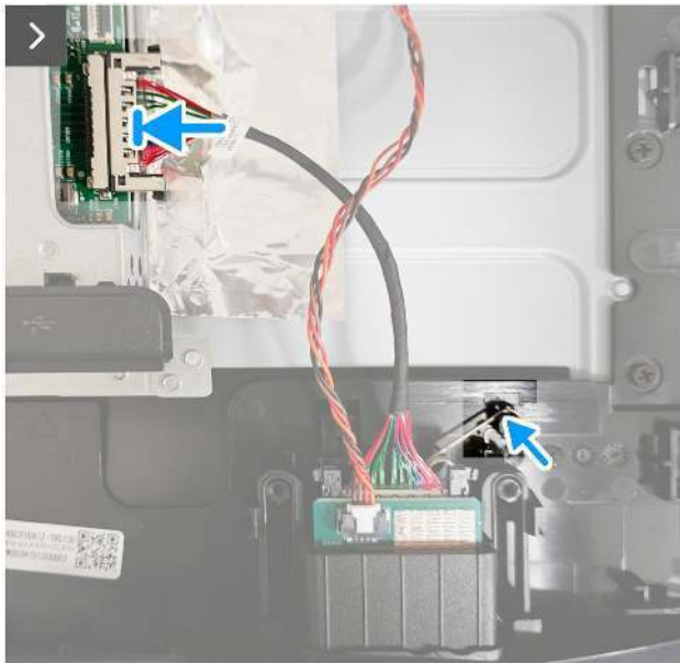
Figure 20. Installing the USB hub
