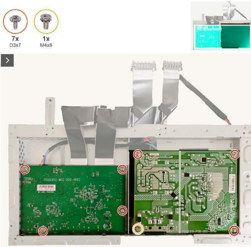
Figure 29. Installing the system board and power board
