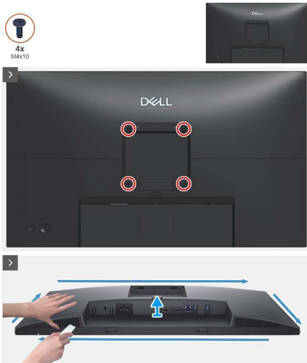
Figure 11. Removing the back cover
