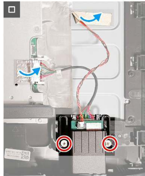
Figure 20. Installing the USB hub
