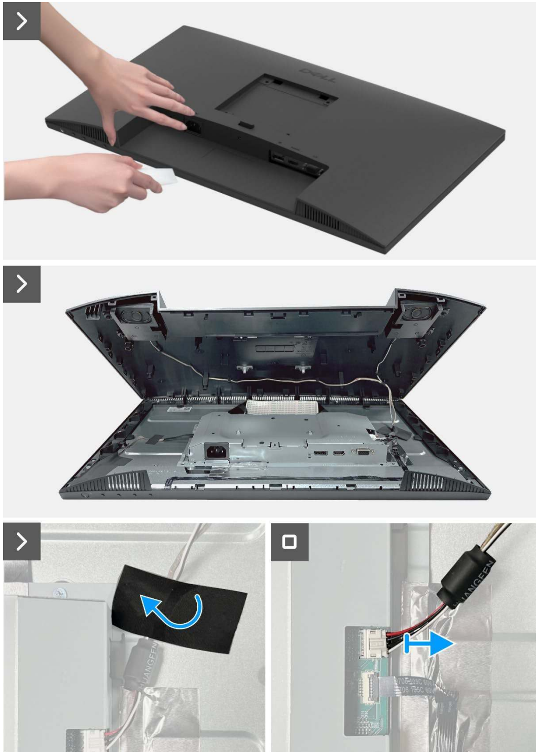
Figure 13. Removing the back cover
