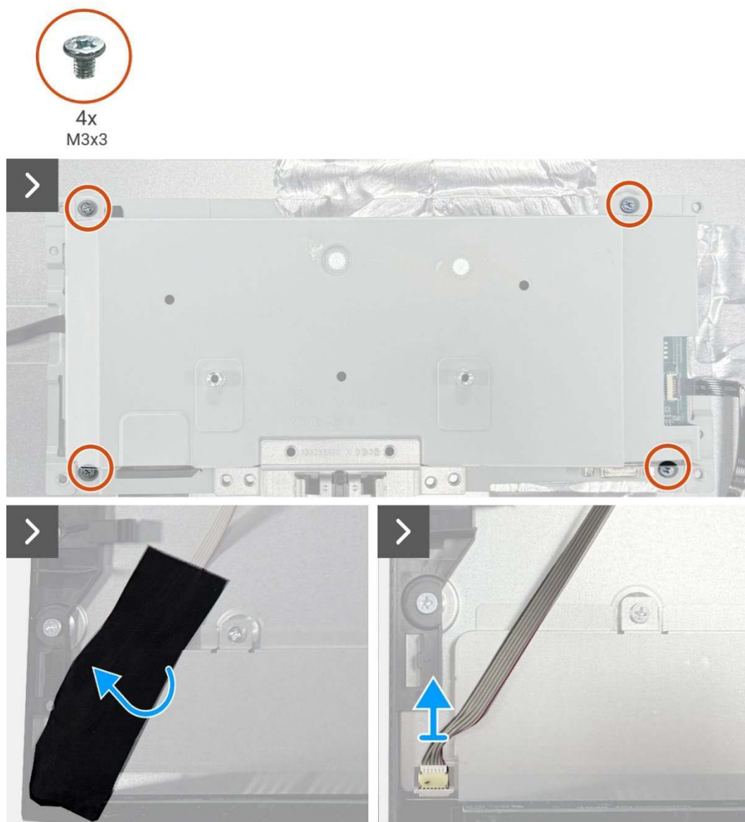
Figure 16. Removing the chassis assembly
