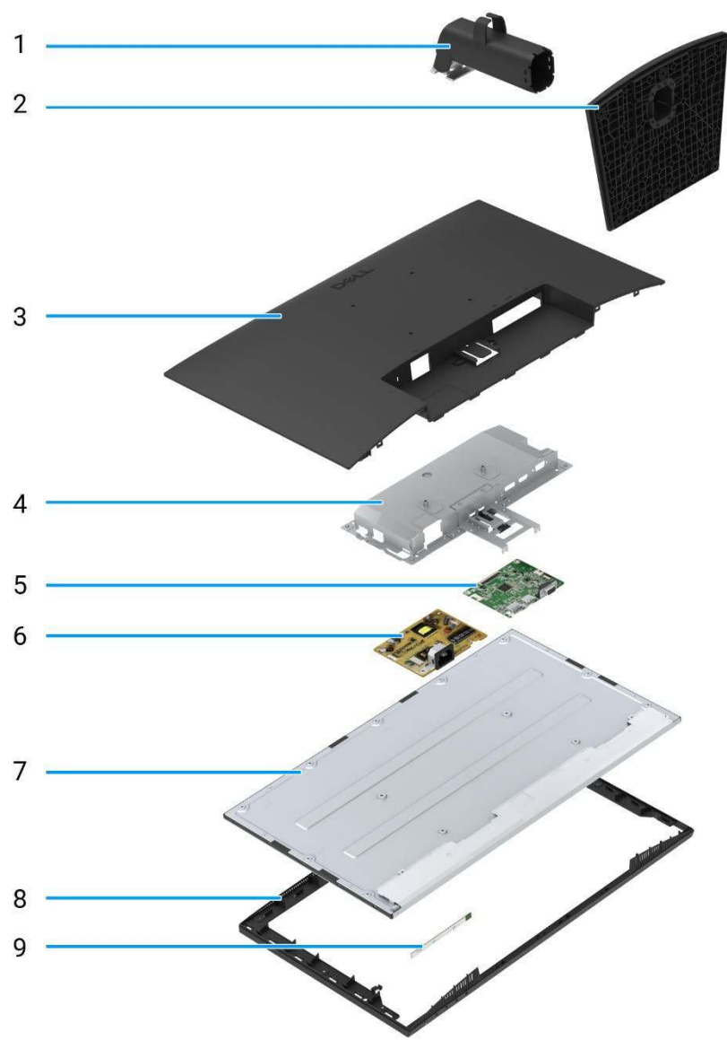
Figure 6. Major components
