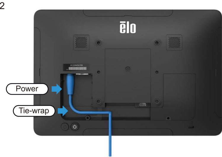
Connect the power cable. The system will power on automatically when plugged in. A tie-wrap (included) can be used to secure the power cable from accidental removal.
