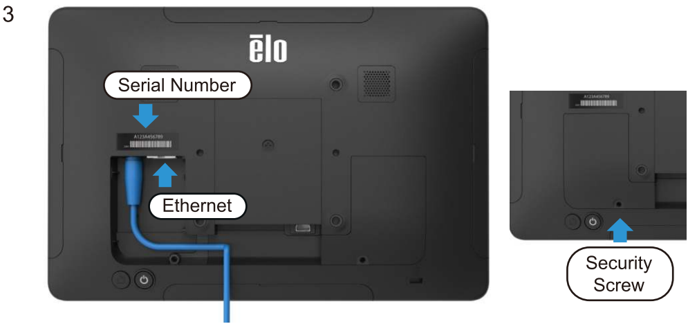
Connect an Ethernet cable now (or setup WiFi later). Once all cables are connected, reinstall the cable over and secure with included security screw.
