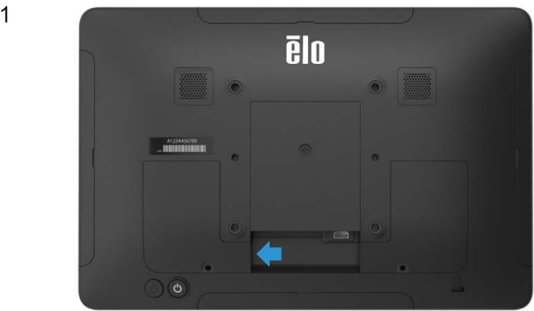
Remove the left side cable cover by lifting upward
