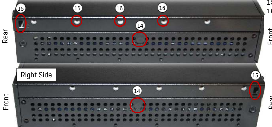
VESA Mount
