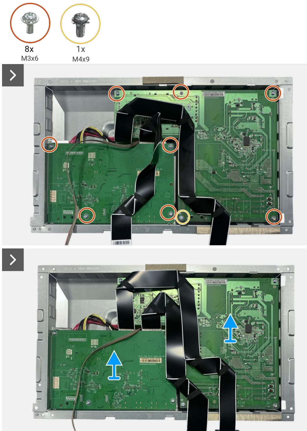
Figure 67. Removing the interface board
