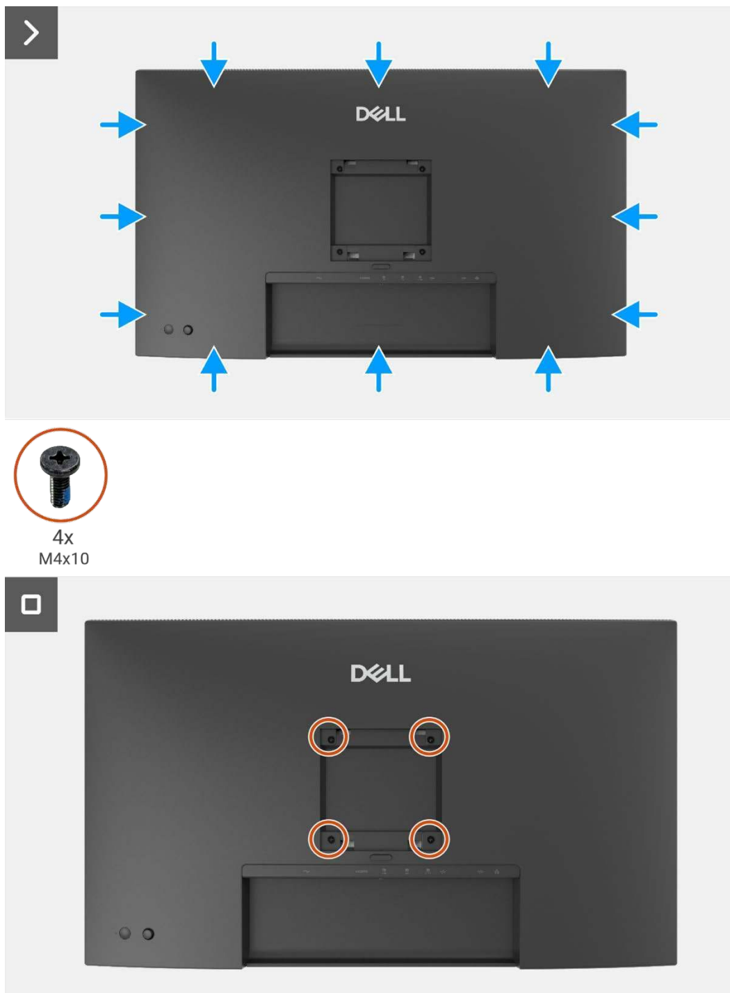
Figure 55. Installing the back cover
