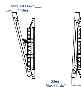
TILT ADJUSTMENT SIDE VIEW
