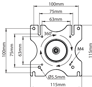
INTERFACE PLATE
