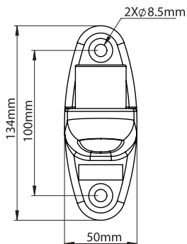
WALL PLATE
