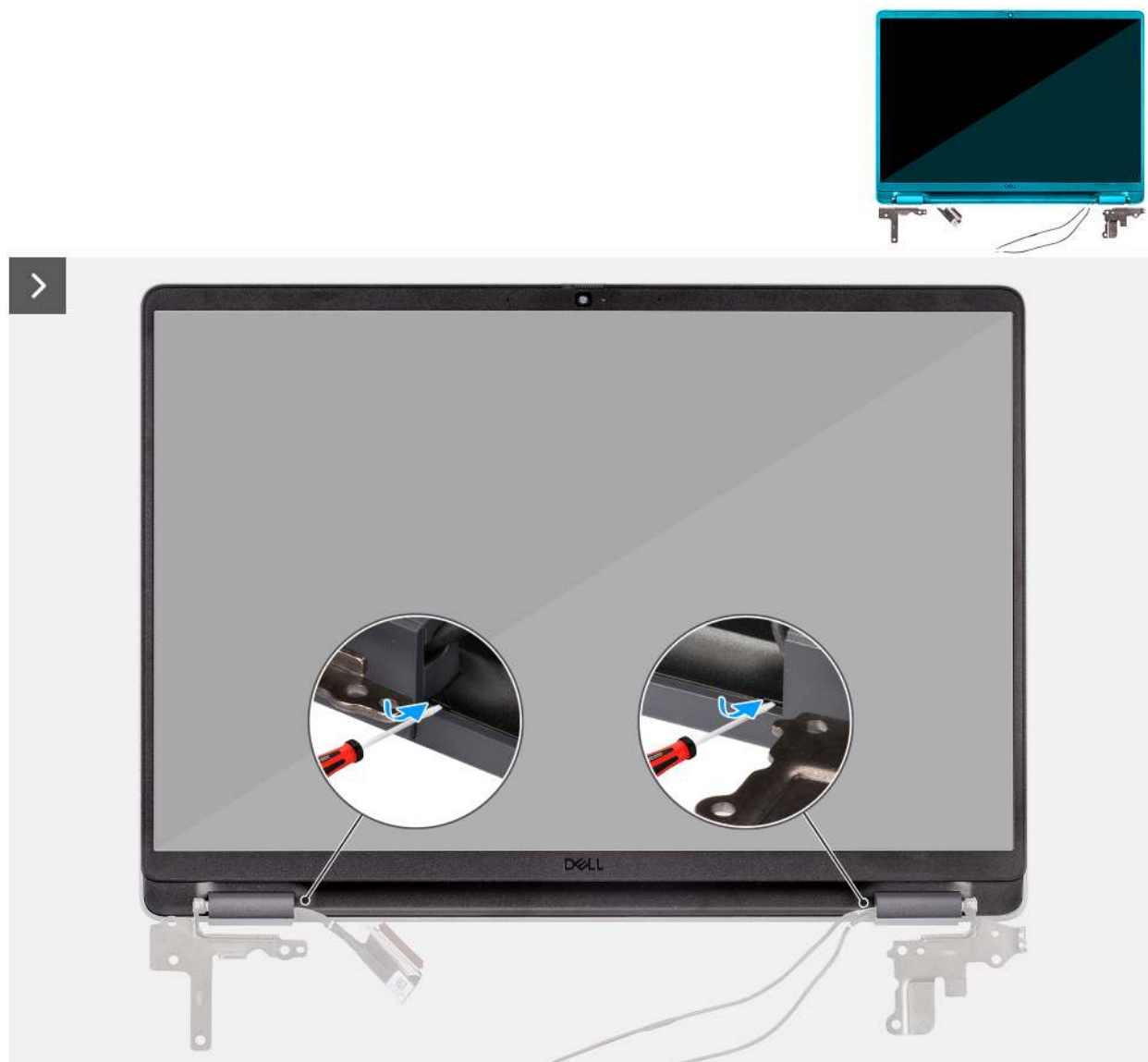
Figure 77. Removing the display bezel
