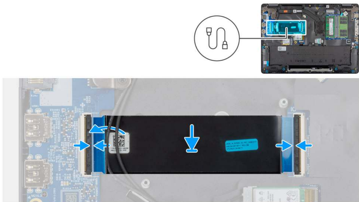
Figure 43. Installing the I/O-board FPC cable
