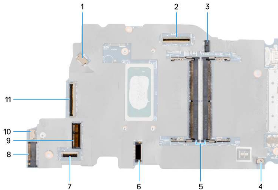
Figure 55. System-board connectors
