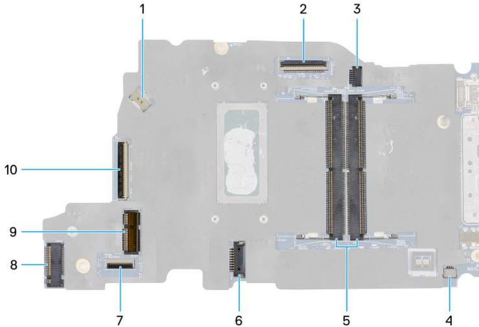
Figure 46. System-board connectors
