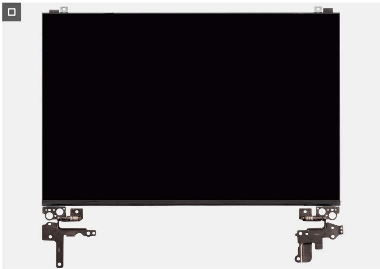
Figure 87. Removing the display-panel assembly
