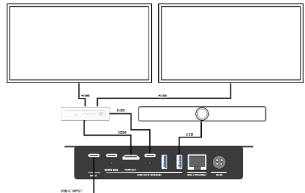
UC-room with BYOD support on Windows-based UC-systems.
