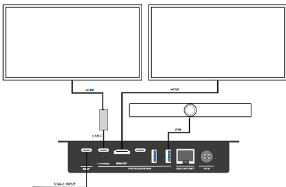
BYOD room with 1 or 2 x4k displays and USB2 and USB 3 device support.
