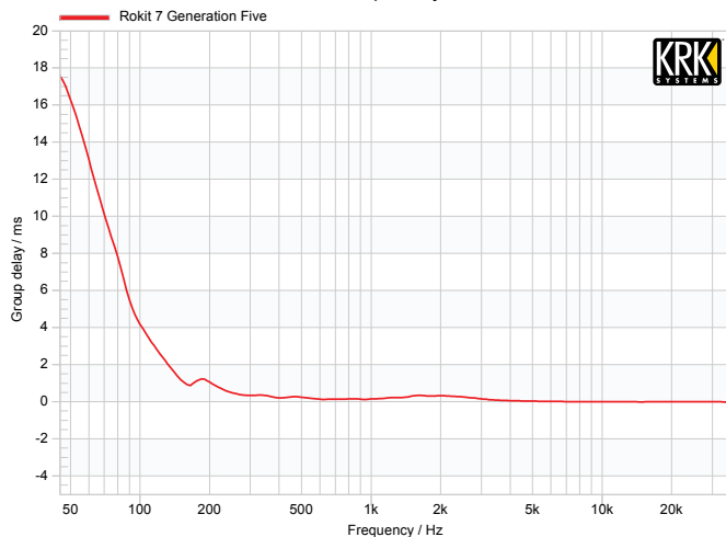
Group Delay
