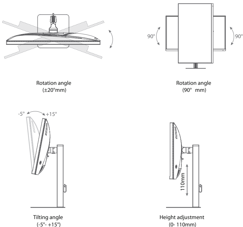
Figure 2-1 Angle Adjustment
