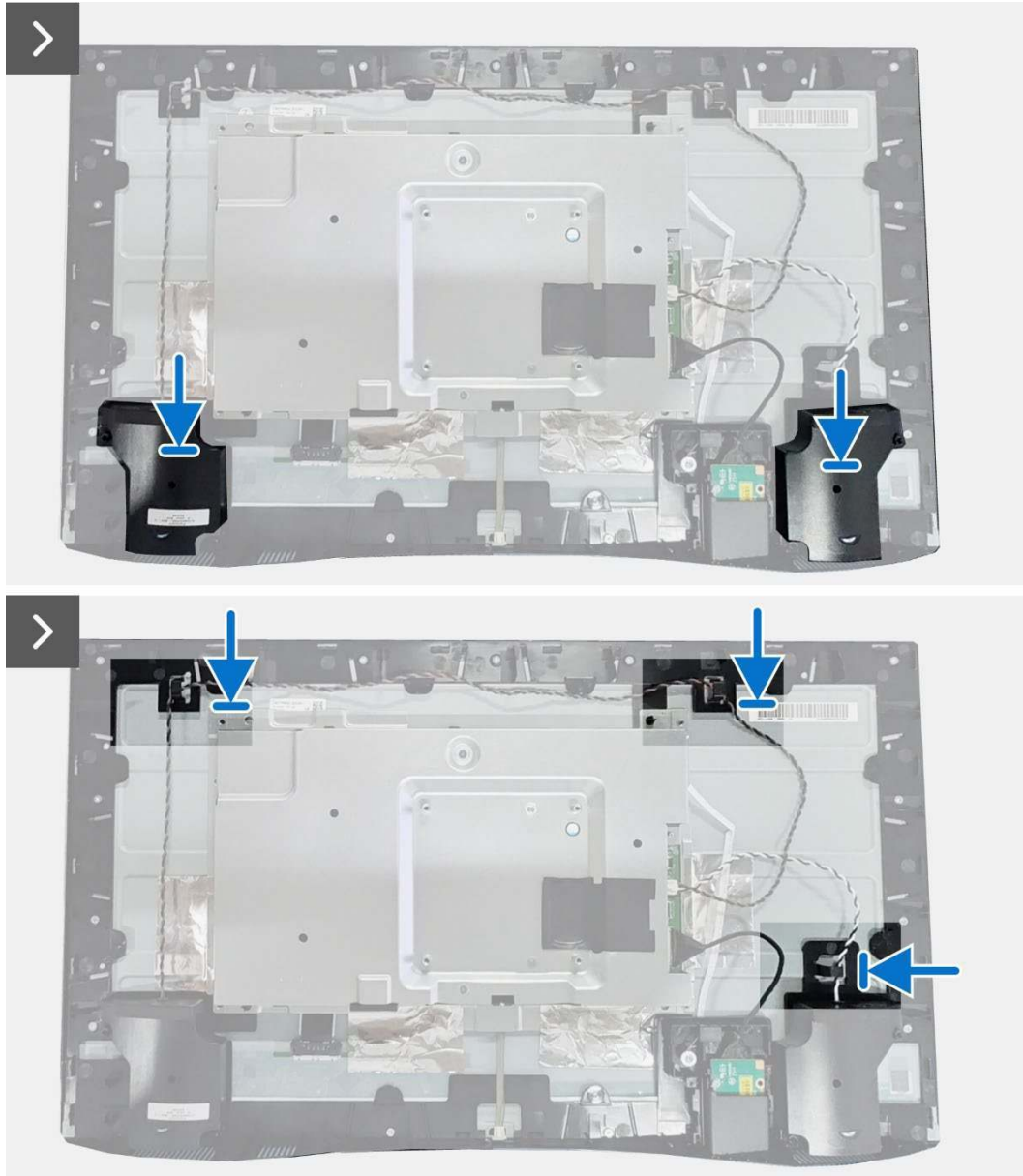
Figure 26. Installing the speakers
