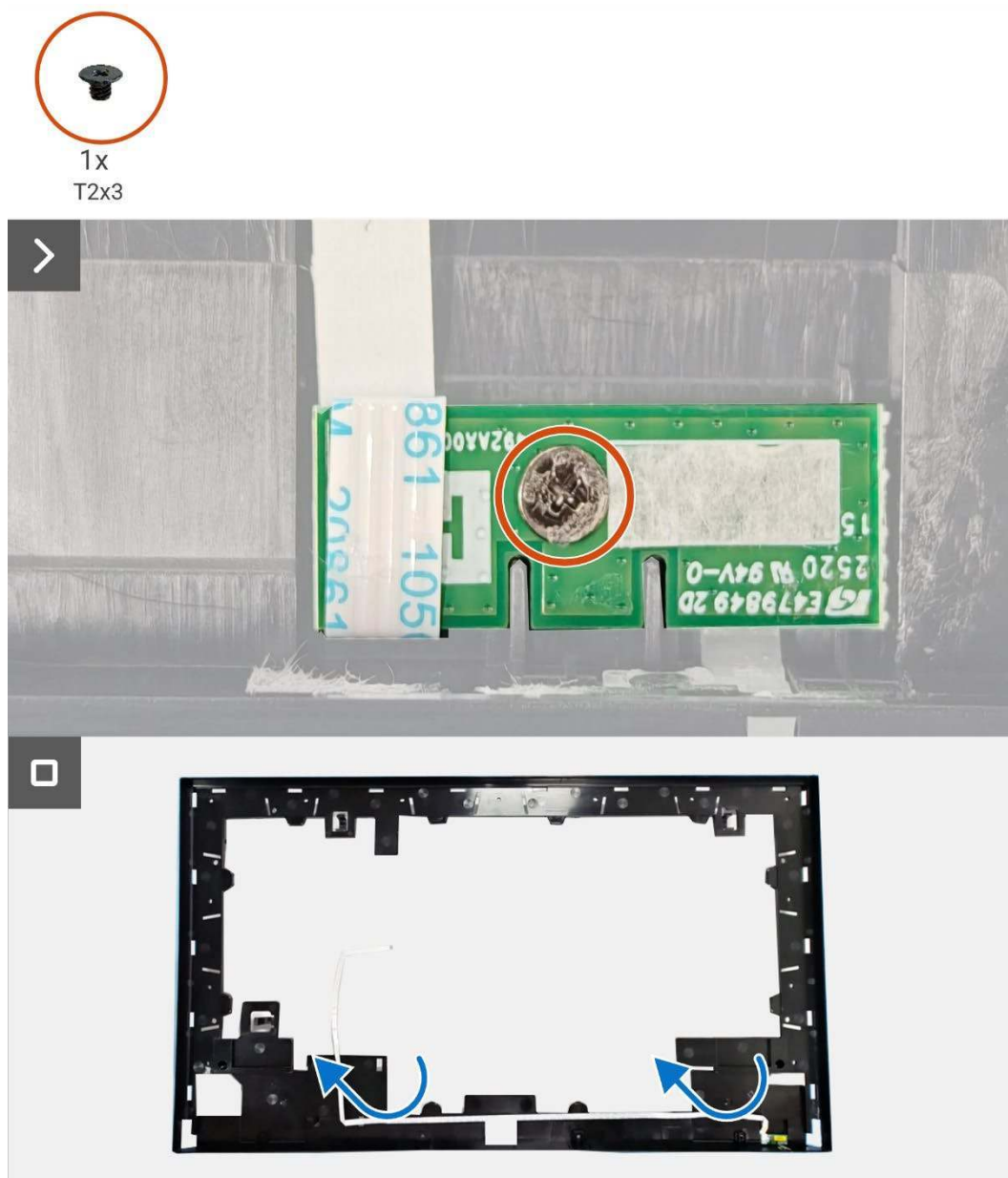
Figure 49. Removing the LED board
